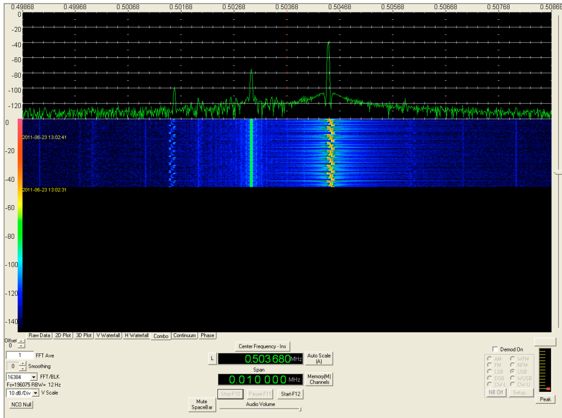
Internal Soundcard (Soundmax HD Audio) almost but not quite trimmed amplitude and phase
